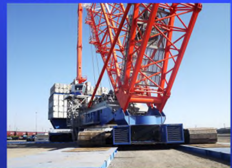
3,000-ton Front Crawler
